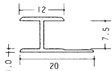
7.5HS (2.73m)
