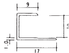
10CS (2.73m)
