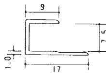
7.5CS (2.73m)
