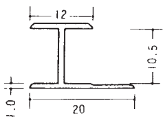
10.5HS (2.73m)
